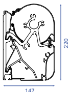
B25 ELITE / PRESTIGE montage murale
